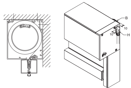
Cable passage B/H without hook profile
